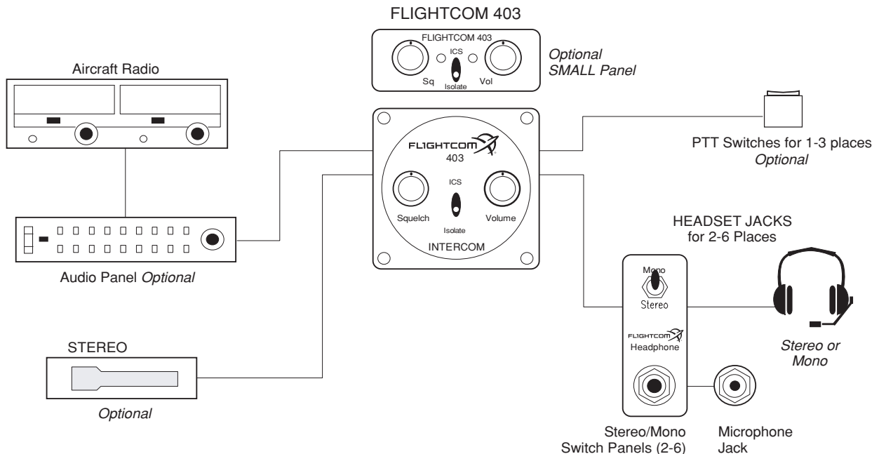
Figure 1 - Model 403/403d Typical Connection Configuration
