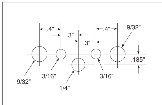
Figure 4 - Drill Templates
